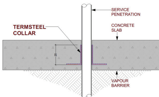
Details for the installation of TermSteel at service penetration.
