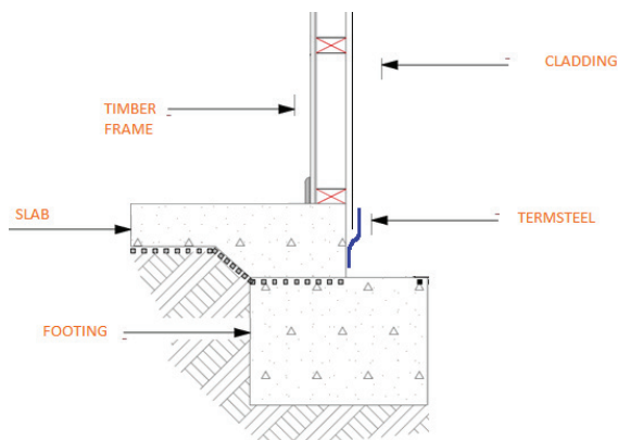
Details for the installation of TermSteel at perimeter from slab to outer wall.
