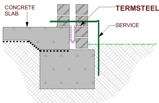
Details for the installation of TermSteel stainless steel mesh at perimeter barrier to walls at Slab-on-ground.
